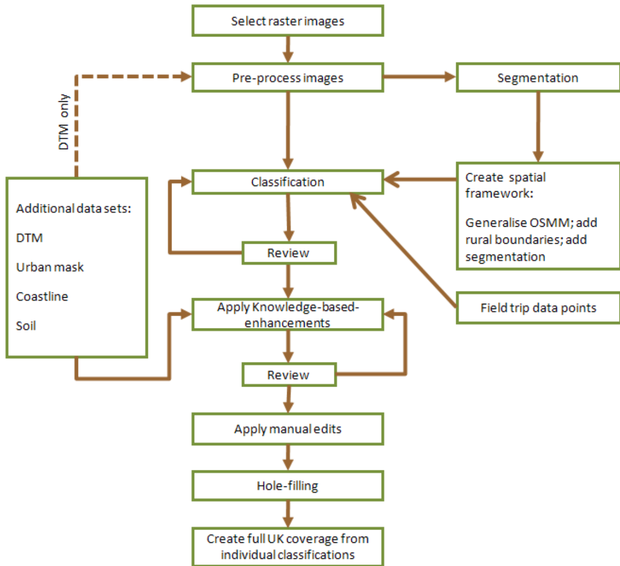
Figure 3.13. Flowchart showing the key stages in the image processing of LCM2007.
