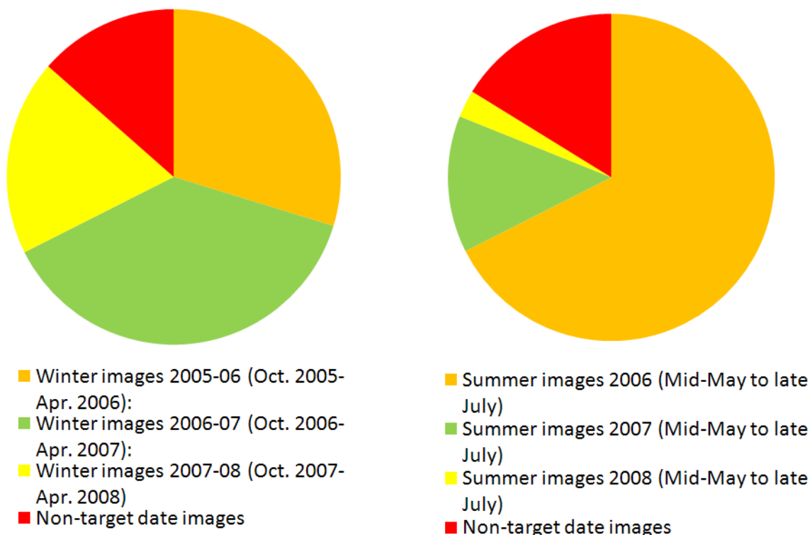
Figure 3.3. Timing of summer and winter images used in LCM2007 composites.
