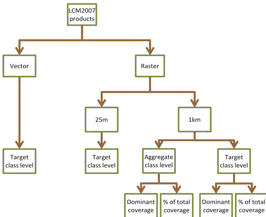
Figure 5.7. Diagram to show the available LCM2007 data products
