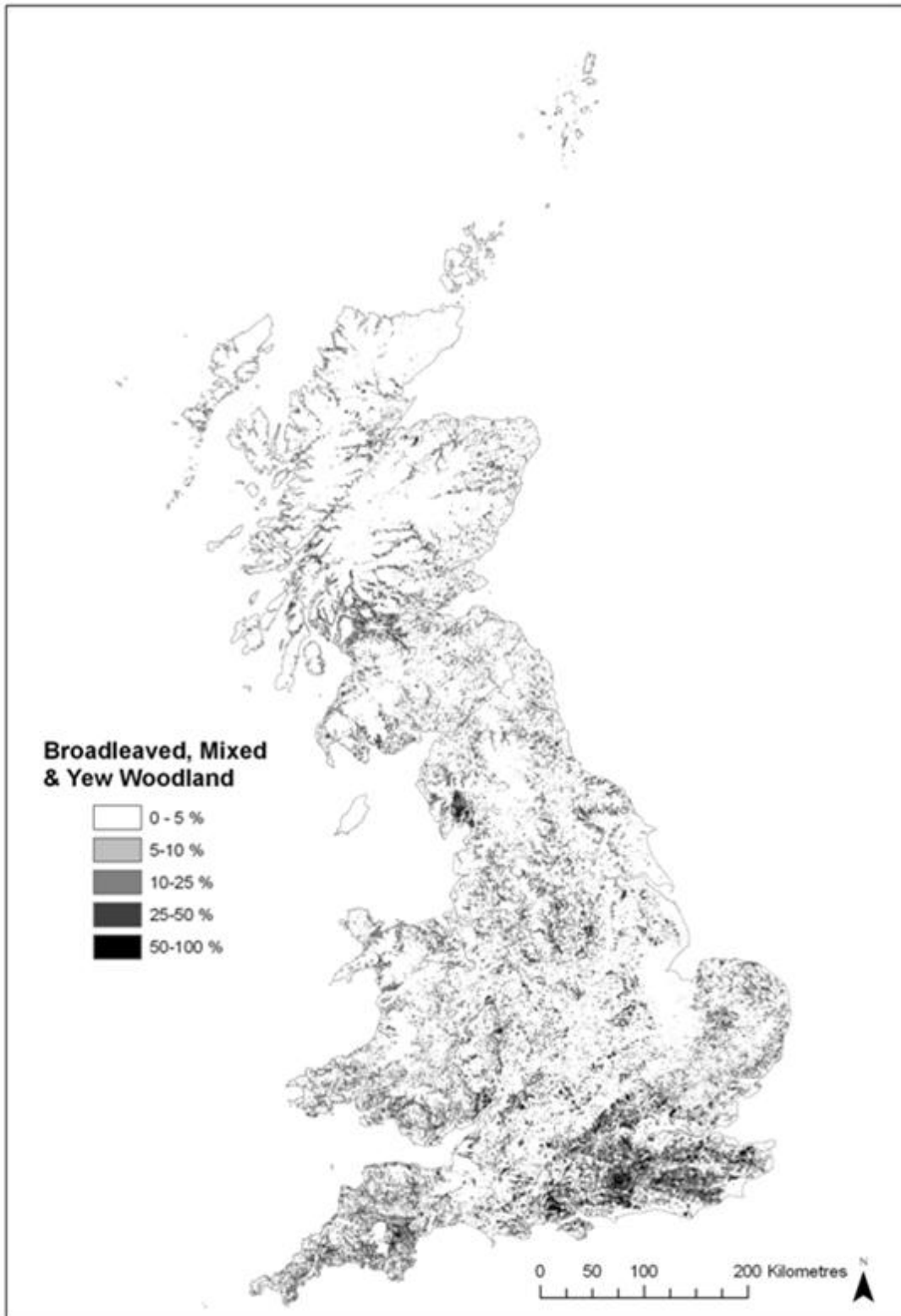
Figure 5.9. Map showing 1km percentage cover raster product for LCM2007 Broadleaved woodland. © NERC (CEH) 2011. Contains Ordnance Survey data © Crown Copyright 2007, 2009. © third-party licensors.
